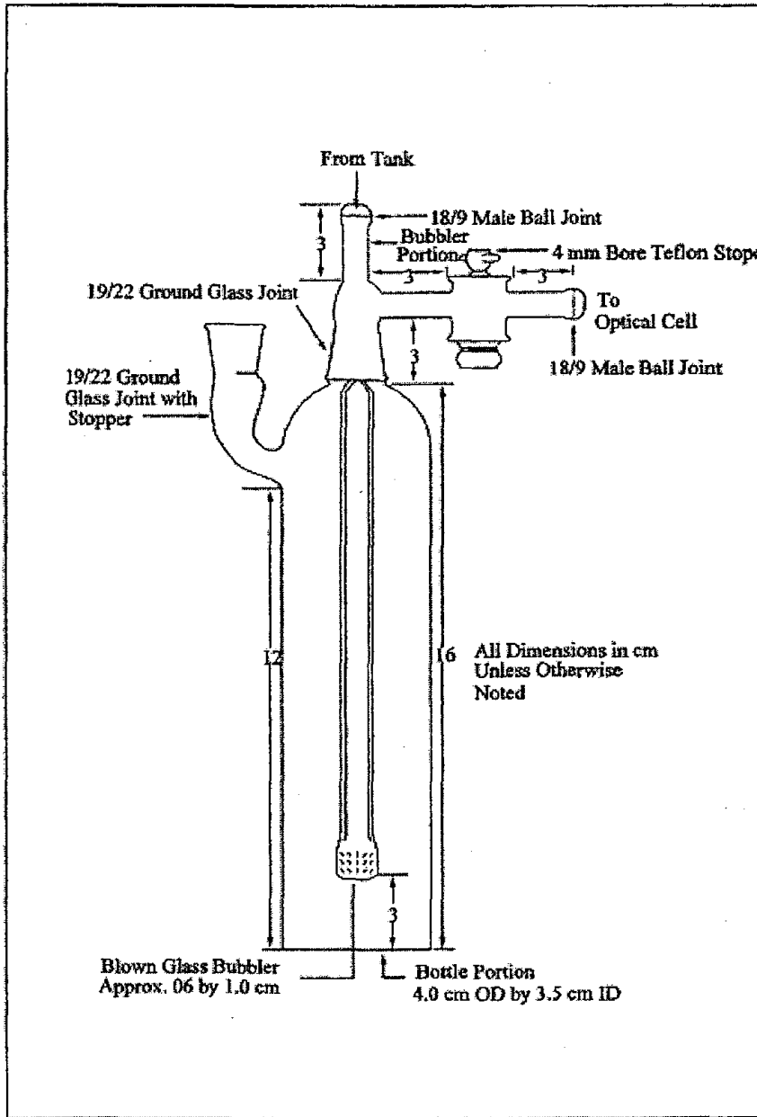
Figure 101-3. Aeration Cell.
