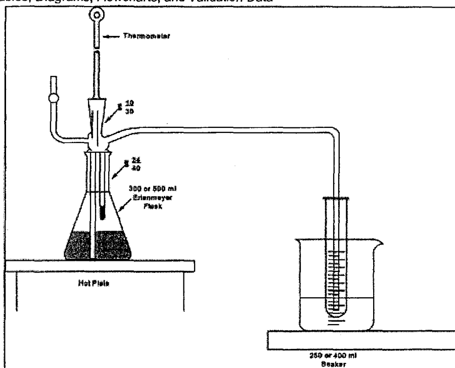
Figure 108C-1. Distillation Apparatus.
