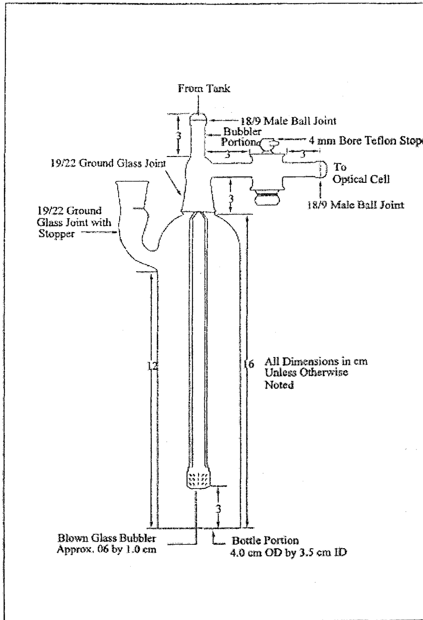
Figure 101-3. Aeration Cell.
