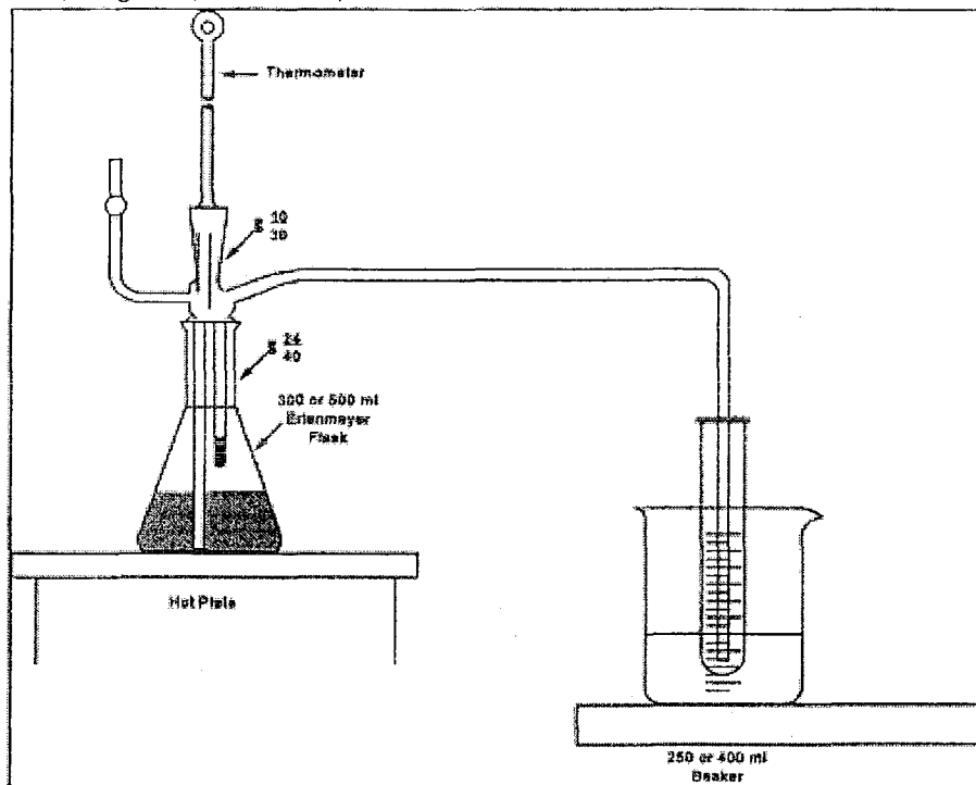
Figure 108C-1. Distillation Apparatus.
