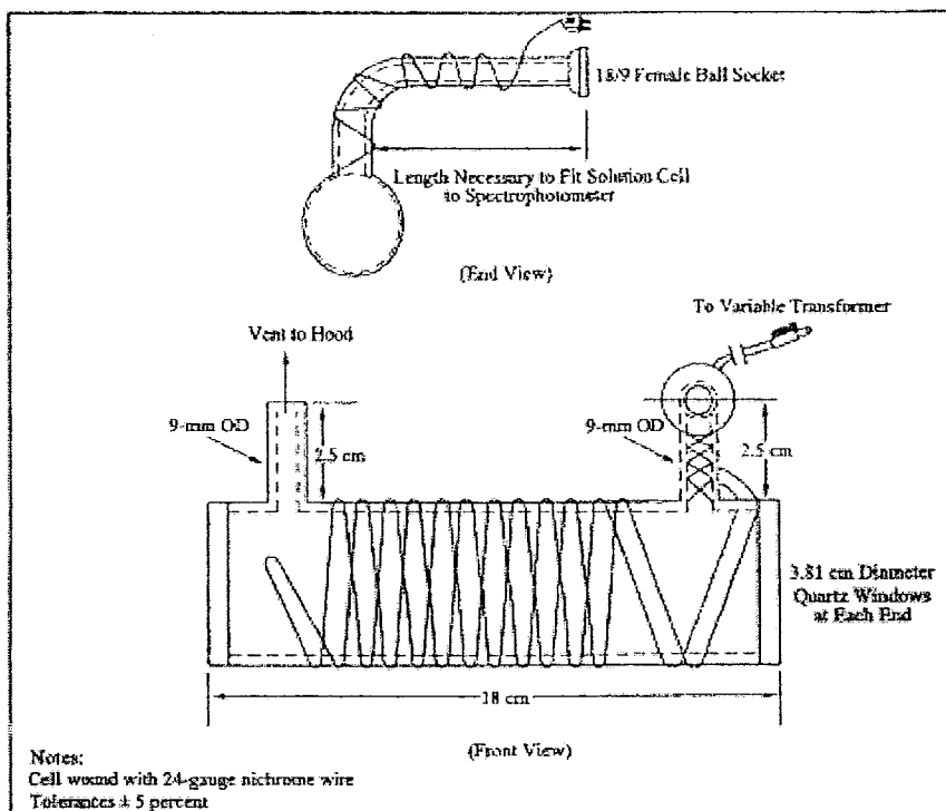
Figure 101-2. Optical Cell.
