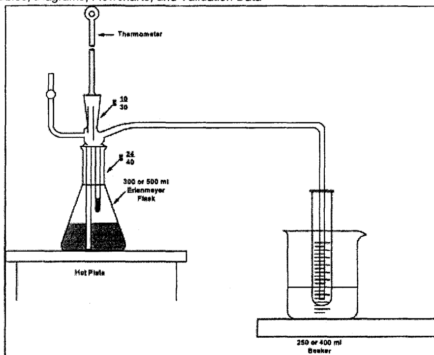
Figure 108C-1. Distillation Apparatus.
