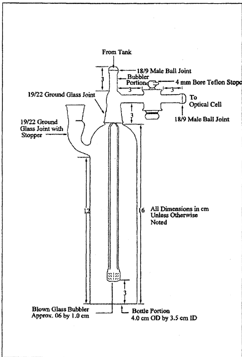
Figure 101-3. Aeration Cell.
