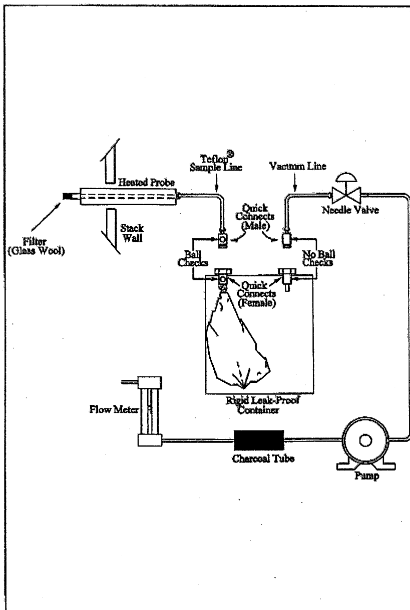
Figure 105-1. Integrated-bag sampling train.
