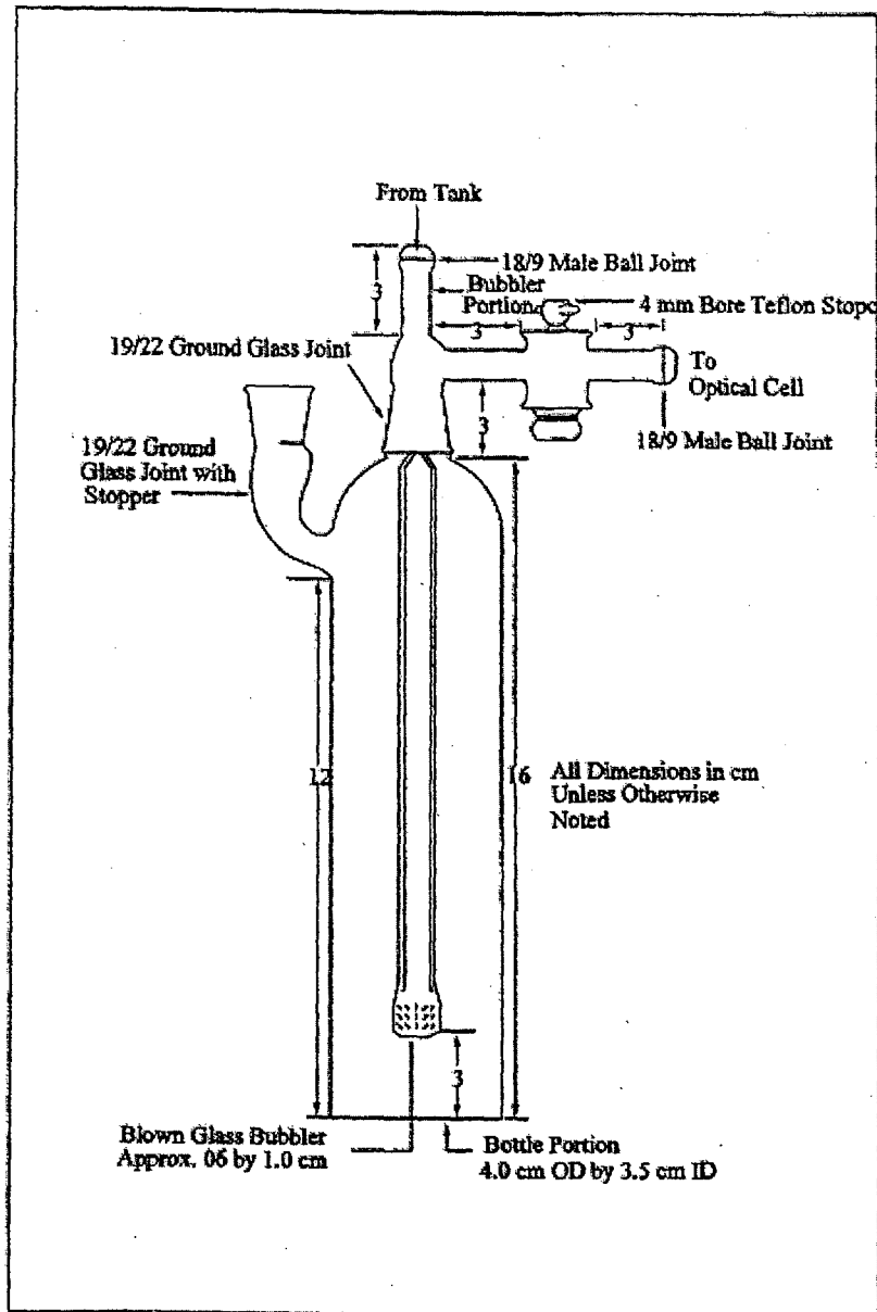
Figure 101-3. Aeration Cell.
