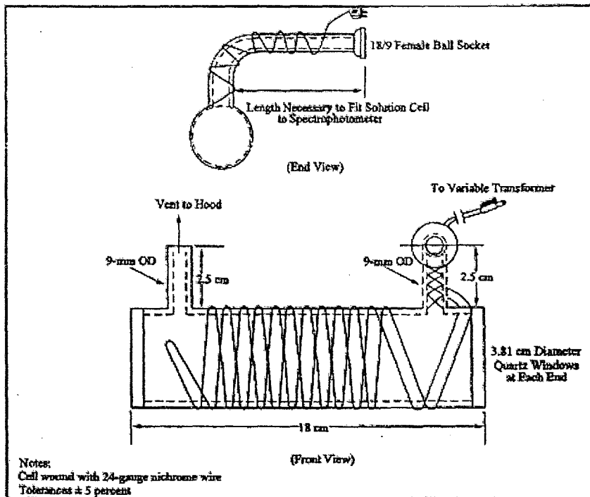
Figure 101-2. Optical Cell.
