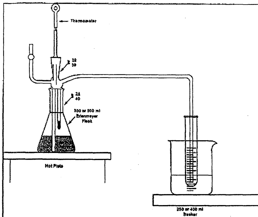
Figure 108C-1. Distillation Apparatus.
