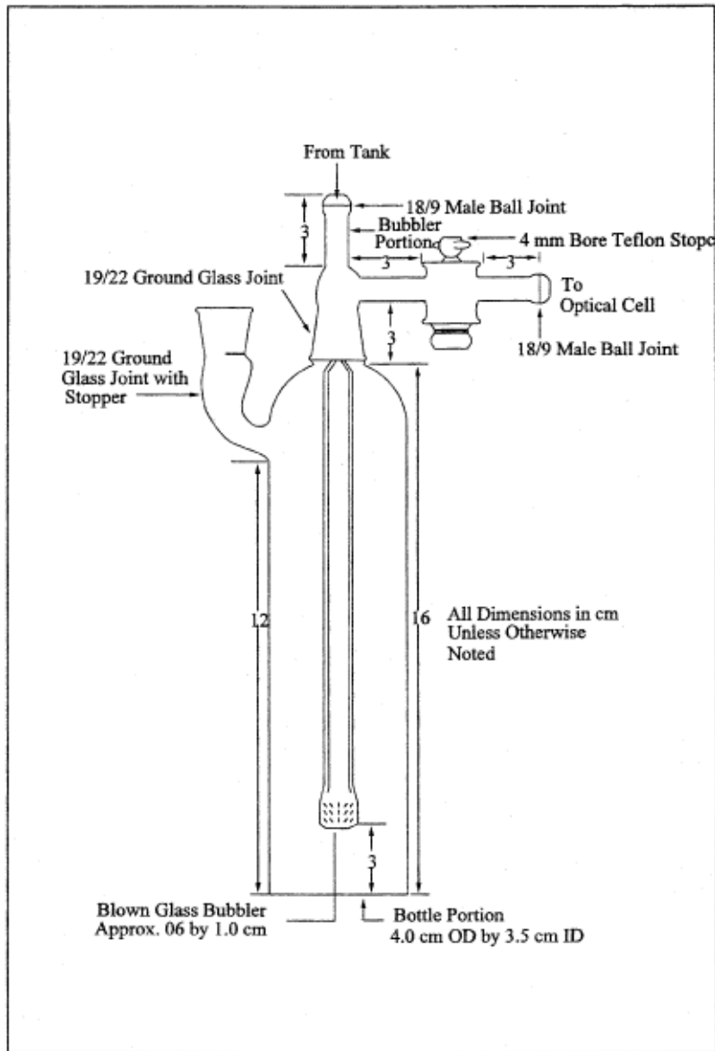
Figure 101-3. Aeration Cell.
