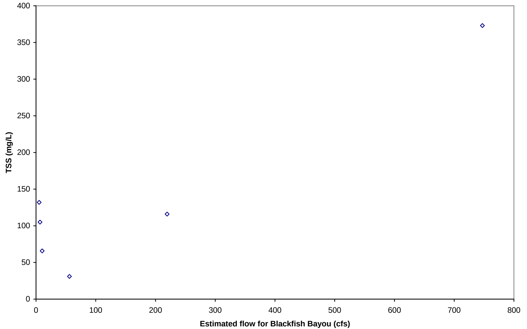
Figure C.24. TSS versus Flow for Blackfish Bayou (FRA0027)
