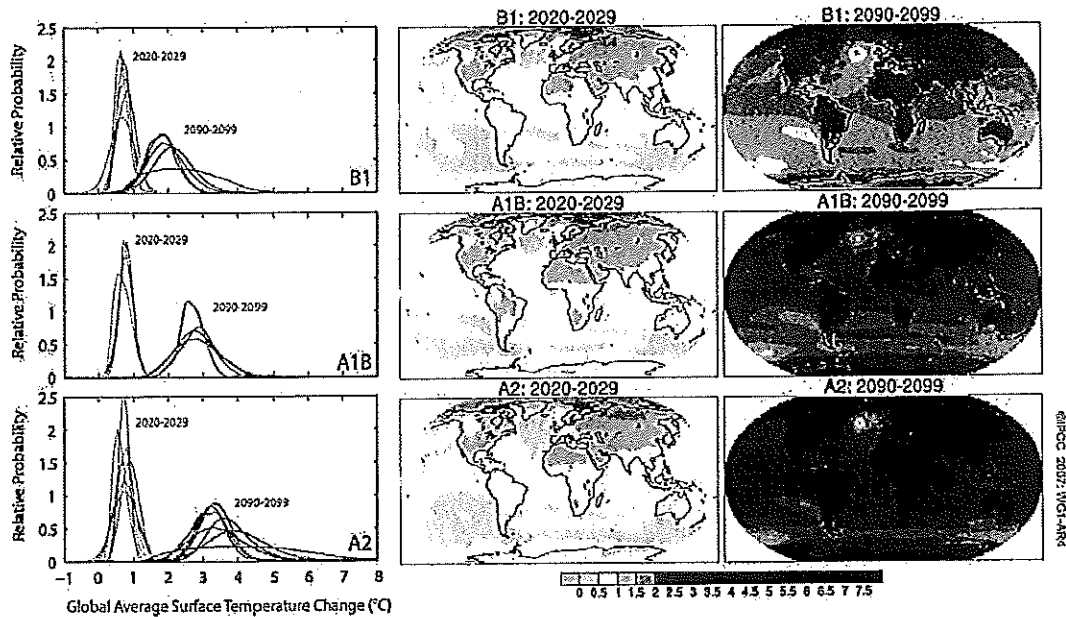
FIGURE SPM-6. Projected surface temperature changes for the early and late 21st century relative to the period 1980–1999. The central and right panels show the Atmosphere-Ocean General Circulation multi-Model average projections for the B1 (top), A1B (middle) and A2 (bottom) SRES scenarios averaged over decades 2020–2029 (center) and 2090–2099 (right). The left panel shows corresponding uncertainties as the relative probabilities of estimated global average warming from several different AOGCM and EMICs studies for the same periods. Some studies present results only for a subset of the SRES scenarios, or for various model versions. Therefore the difference in the number of curves, shown in the left-hand panels, is due only to differences in the availability of results. {Figures 10.8 and 10.28}
