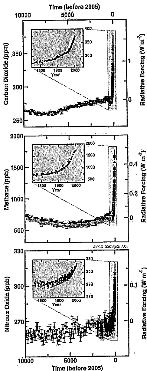
FIGURE SPM-1. Atmospheric concentrations of carbon dioxide, methane and nitrous oxide over the last 10,000 years (large panels) and since 1750 (inset panels). Measurements are shown from ice cores (symbols with different colours for different studies) and atmospheric samples (red lines). The corresponding radiative forcings are shown on the right hand axes of the large panels. {Figure 6.4}
