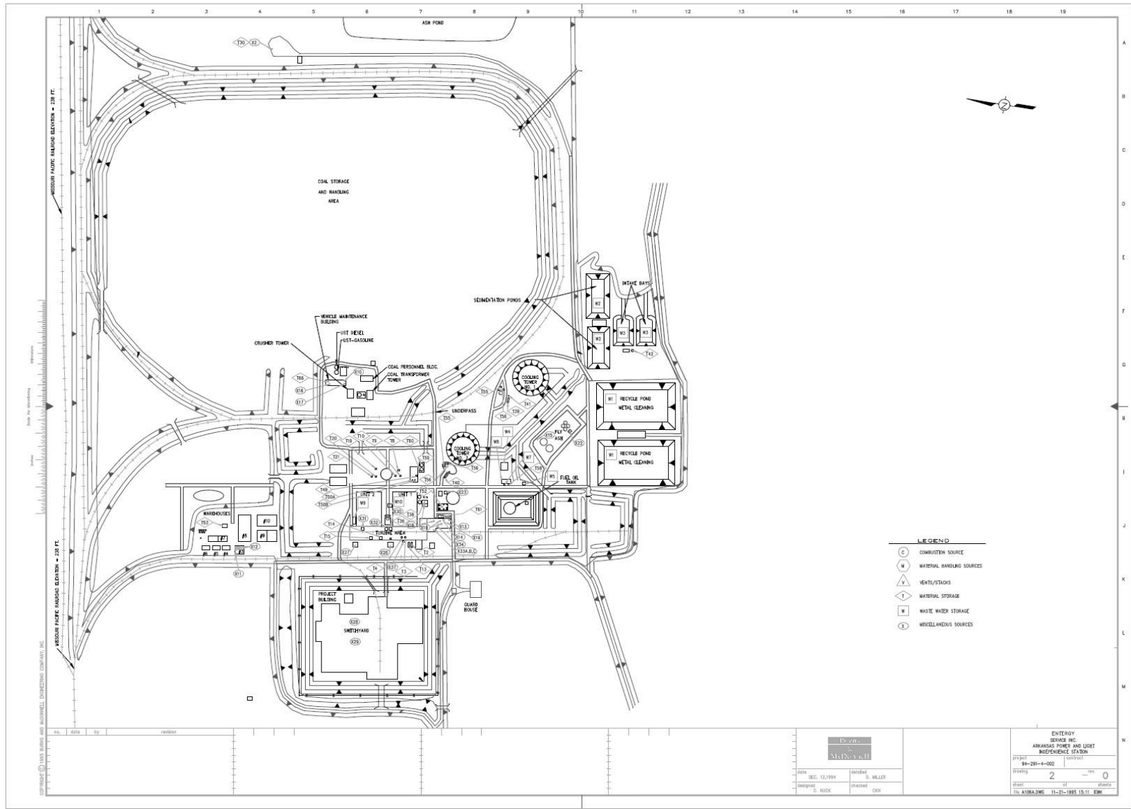
Figure 2-1 Independence Station Site Plan
