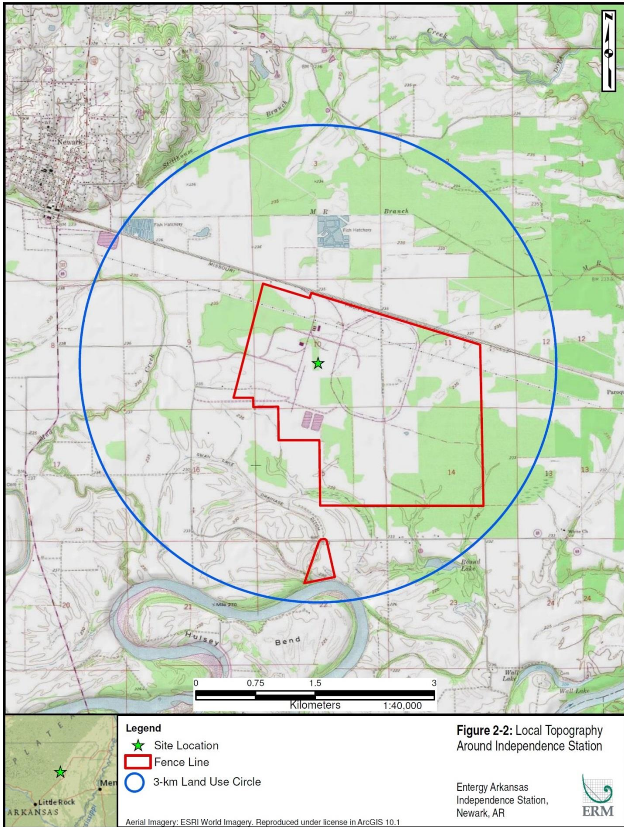
Figure 2-2 Independence Station Local Topography
