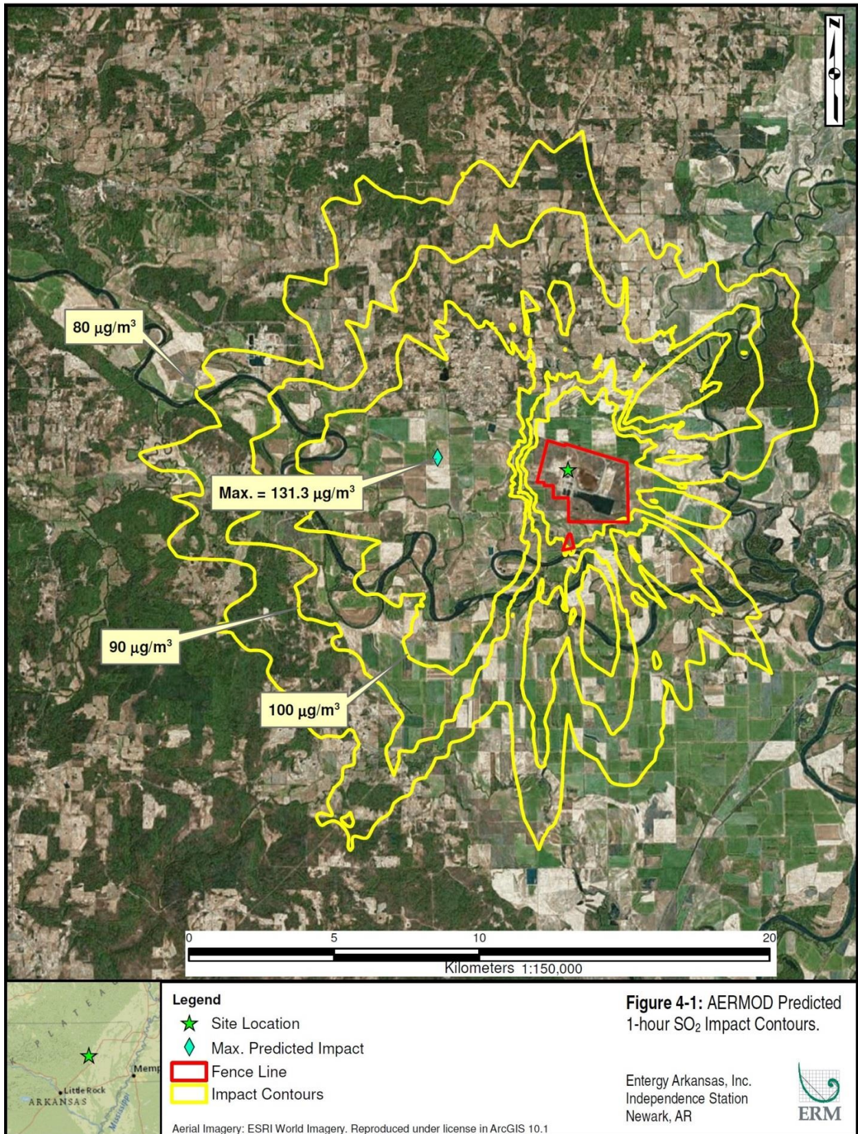
Figure 4-1 Independence Station 1-hour SO 2 Impact Contours
