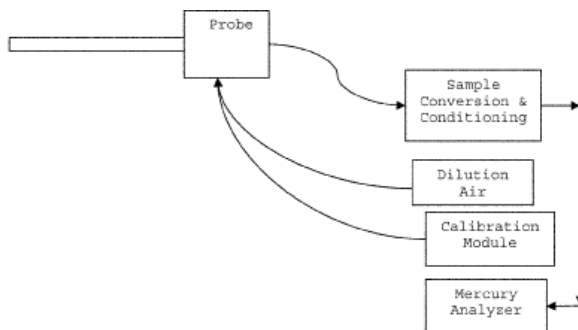
FIGURE A-1. TYPICAL MERCURY CEMS
