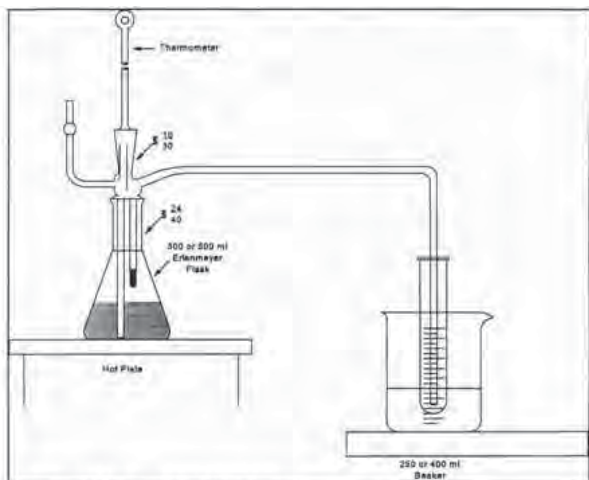
Figure 108C-1. Distillation Apparatus.
