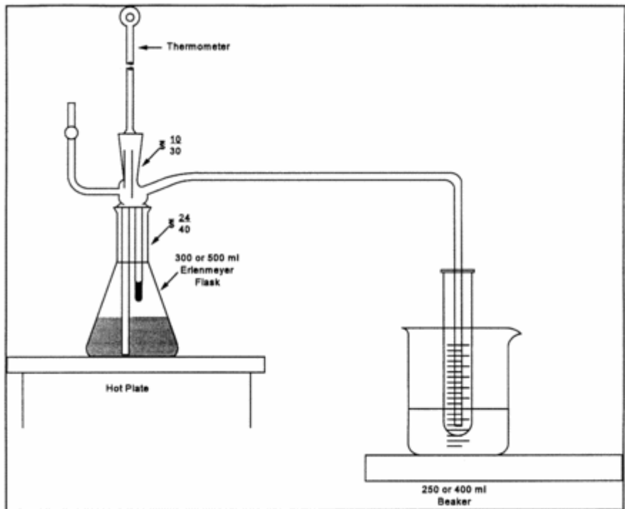
Figure 108C-1. Distillation Apparatus.
