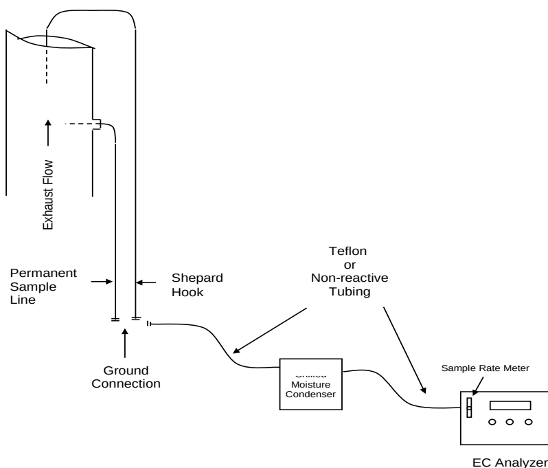
Figure 2 Calibration Assembly
