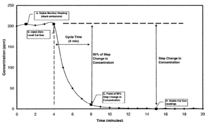
Figure 6b. Downscale Cycle Time Test
