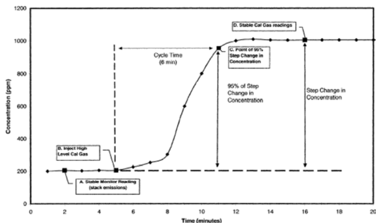
Figure 6a. Upscale Cycle Time Test
