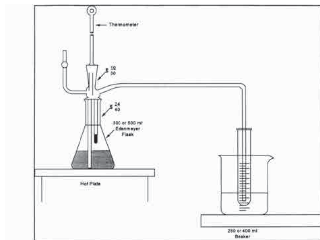
Figure 108C-1. Distillation Apparatus.
