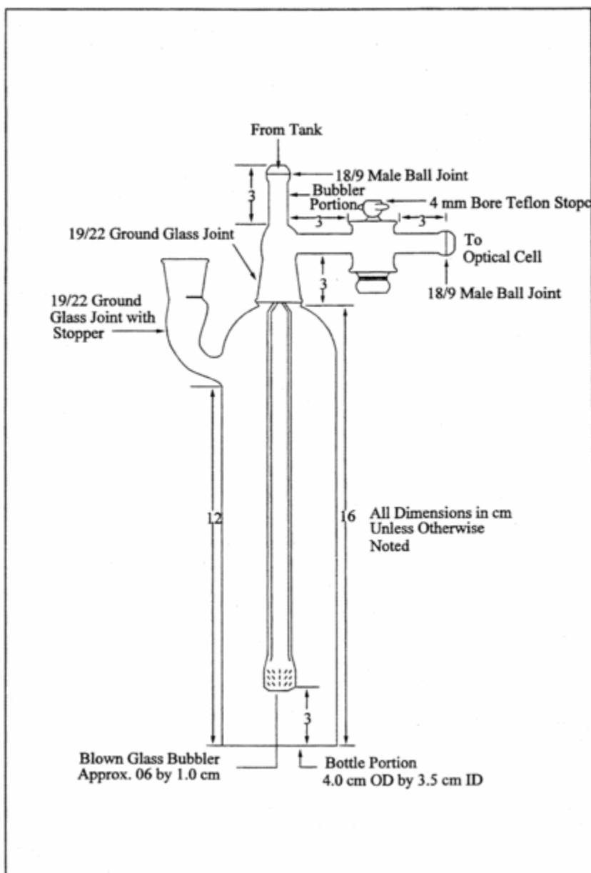
Figure 101-3. Aeration Cell.
