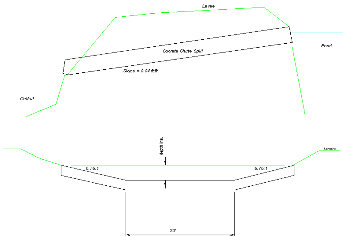
Schematic of Concrete Chute Spillway
