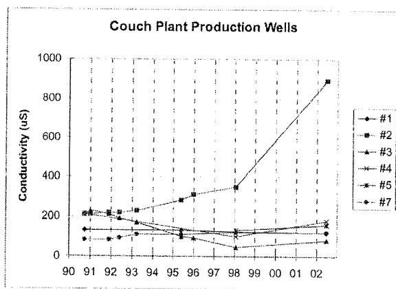
Figure 8.1. Time series plots for conductivity, chlorides and iron from Couch wells 2, 3, 4, 5, and 7.
