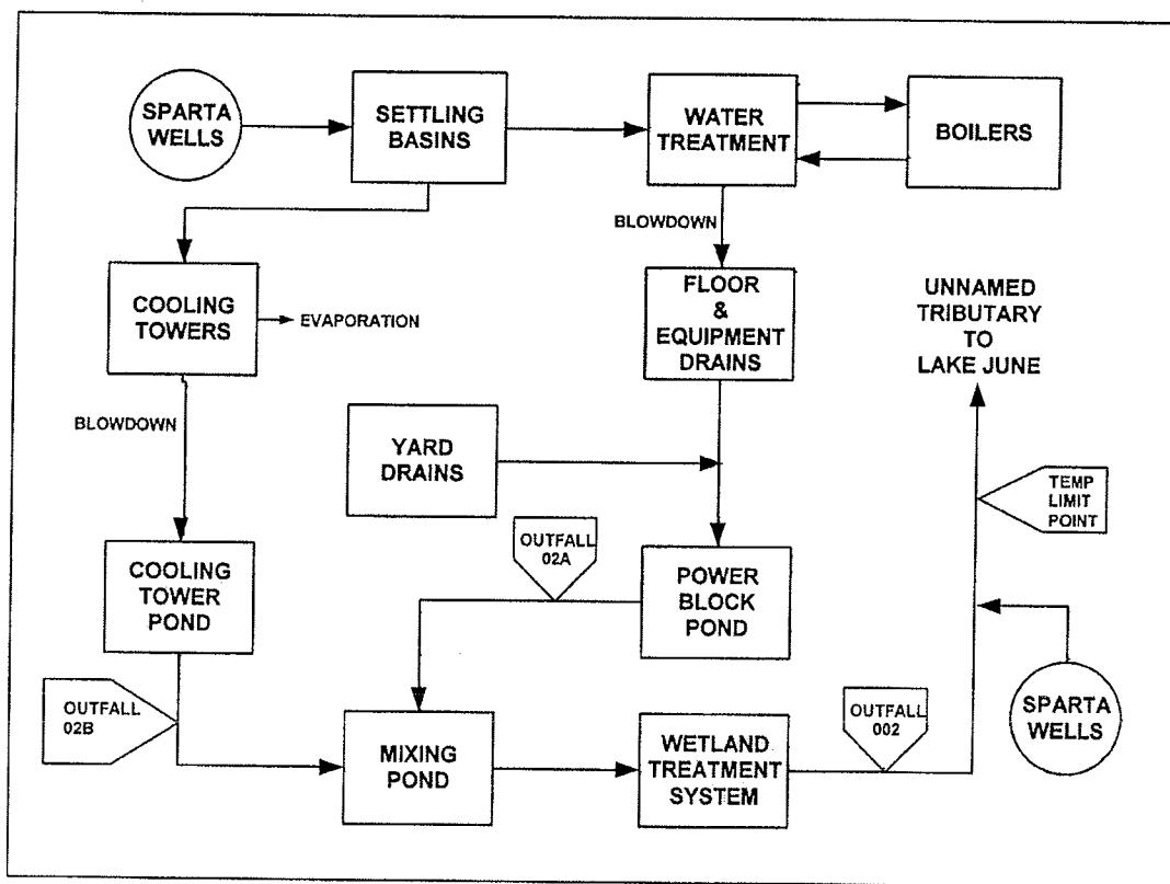
Figure 2.1. Flow diagram of Couch Plant.
