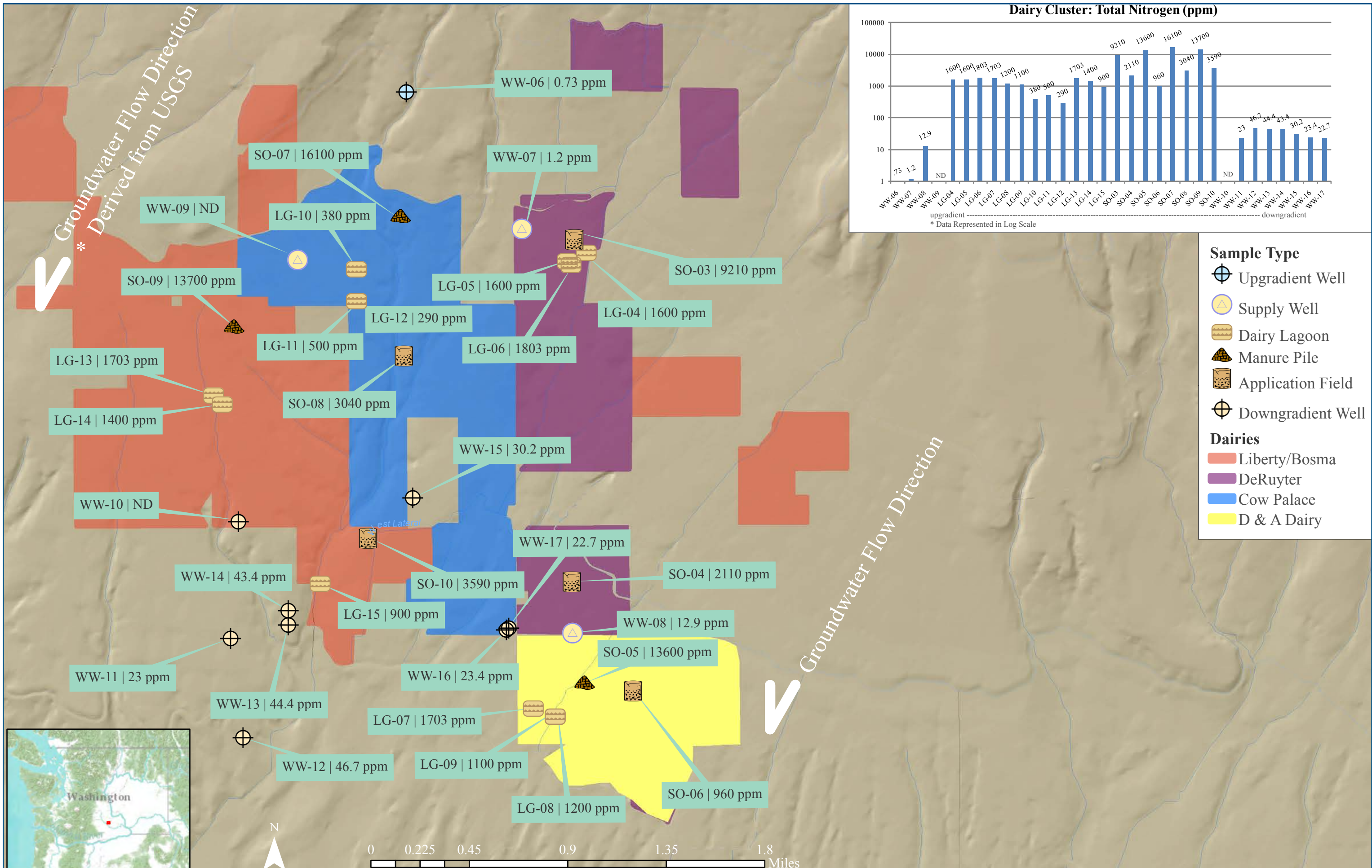
Figure 15: Dairy Cluster: Total Nitrogen Concentrations in Water Wells, Lagoons, Manure Piles, and Application Fields
