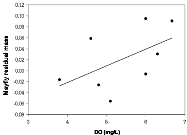
Figure 2. Linear regression between DO and body condition of low-DO-sensitive mayfly larvae from isolated pools in the Alum Fork of the Saline River (summer 2002). Measurements of DO were averaged across months (June-July). From Love et al. (2005).
