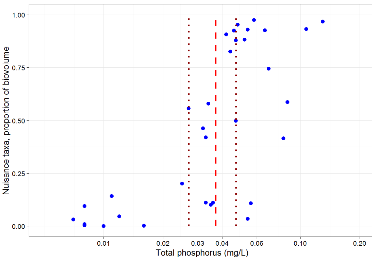
Figure 20. Two-year mean TP (April 2014-2016) vs. mean nuisance taxa proportion from events 1, 3, 5, 6, 9, and 12. The dashed red line corresponds to 0.037 mg/L TP, whereas the dotted lines correspond to 0.027 and 0.047 mg/L TP, respectively.
