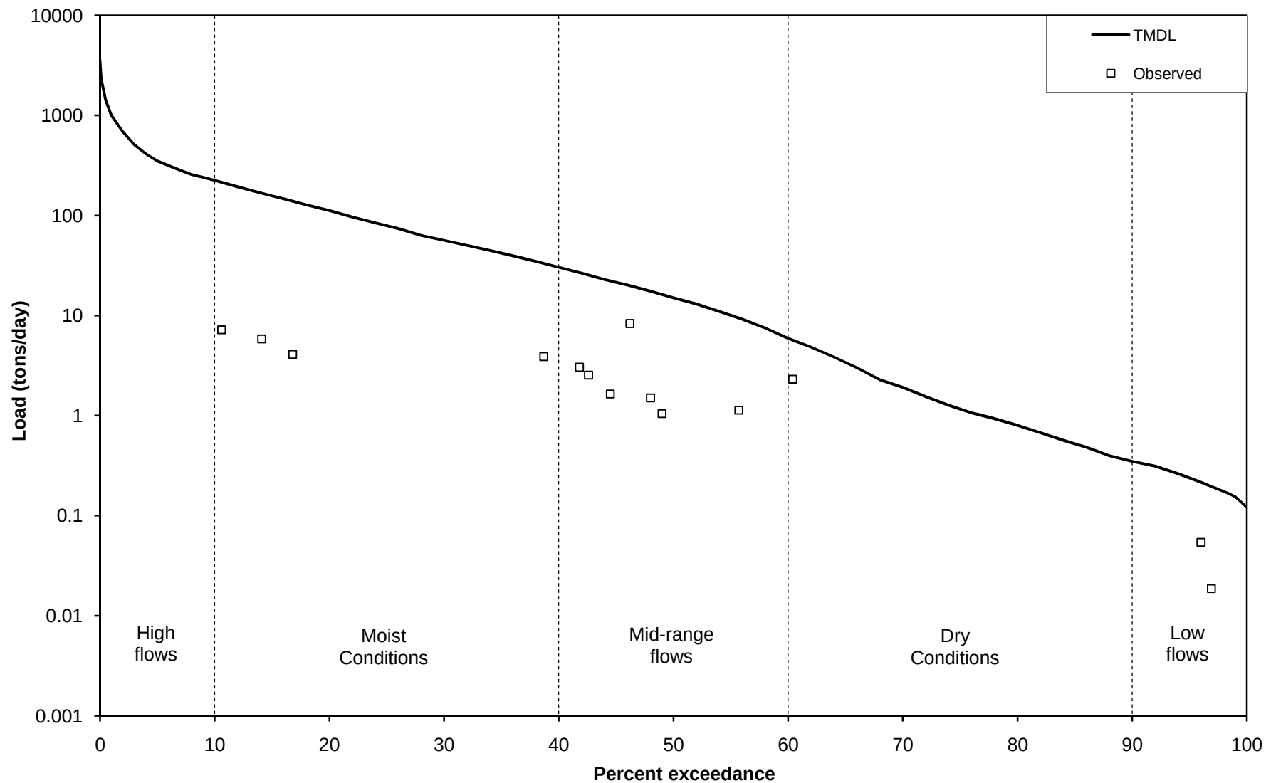
Figure L.4 Sulfate Load Duration Curve for Big Creek Reach 11140203-023
