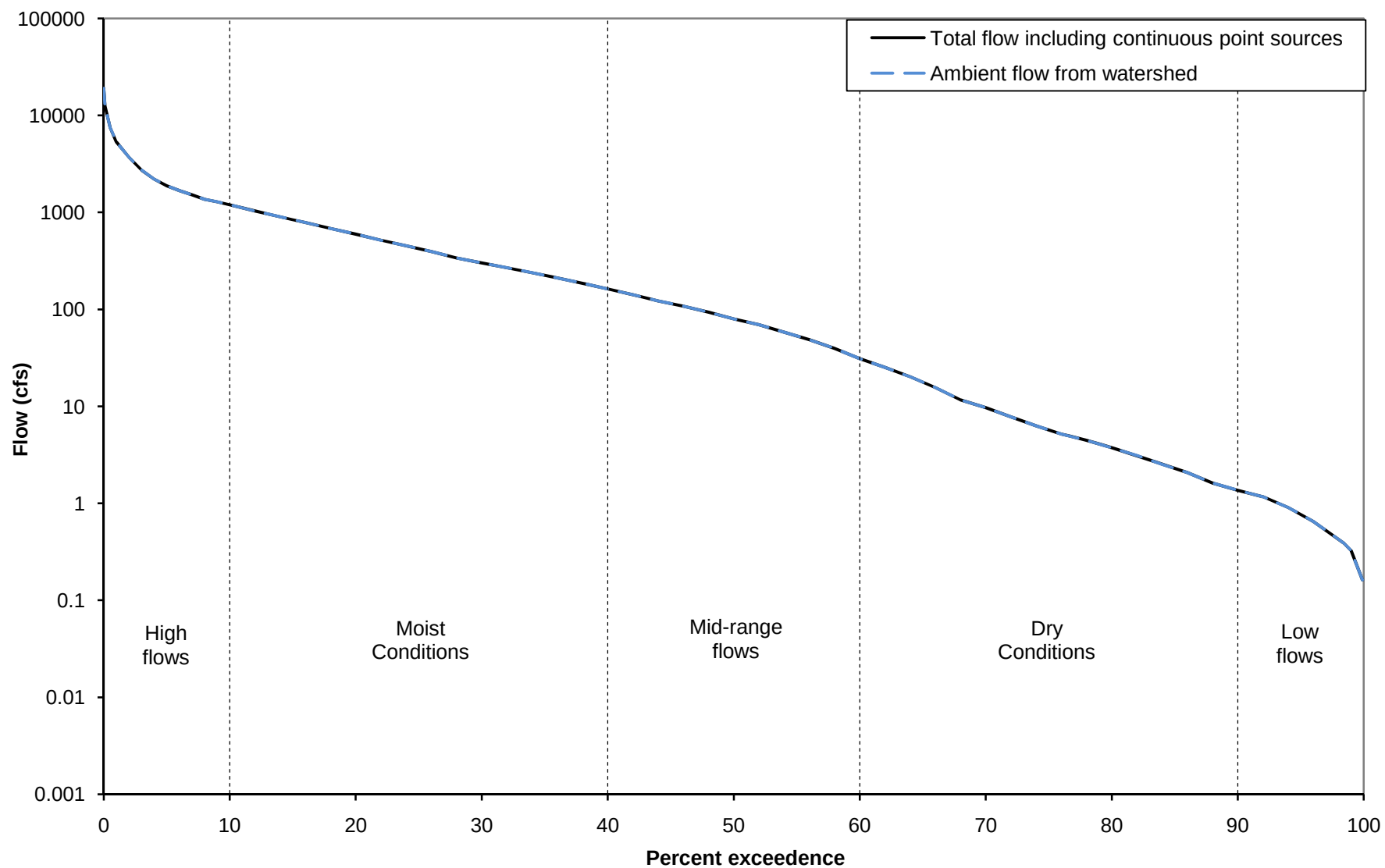
Figure M.1 Flow Duration Curve for Dorcheat Bayou Reach 11140203-22
