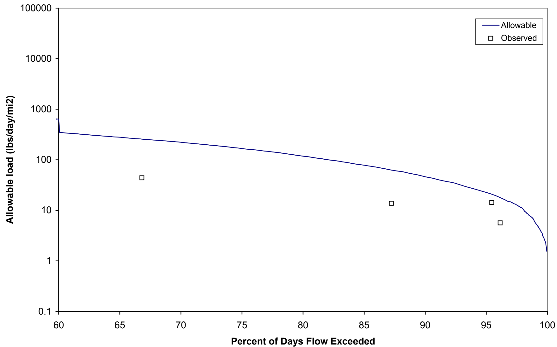
Figure F.3. Base flow Load Duration Curve for Tyronza River (FRA0033)
