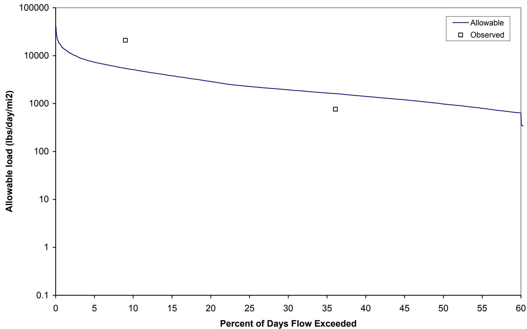
Figure F.2. Storm-flow Load Duration Curve for Tyronza River (FRA0033)
