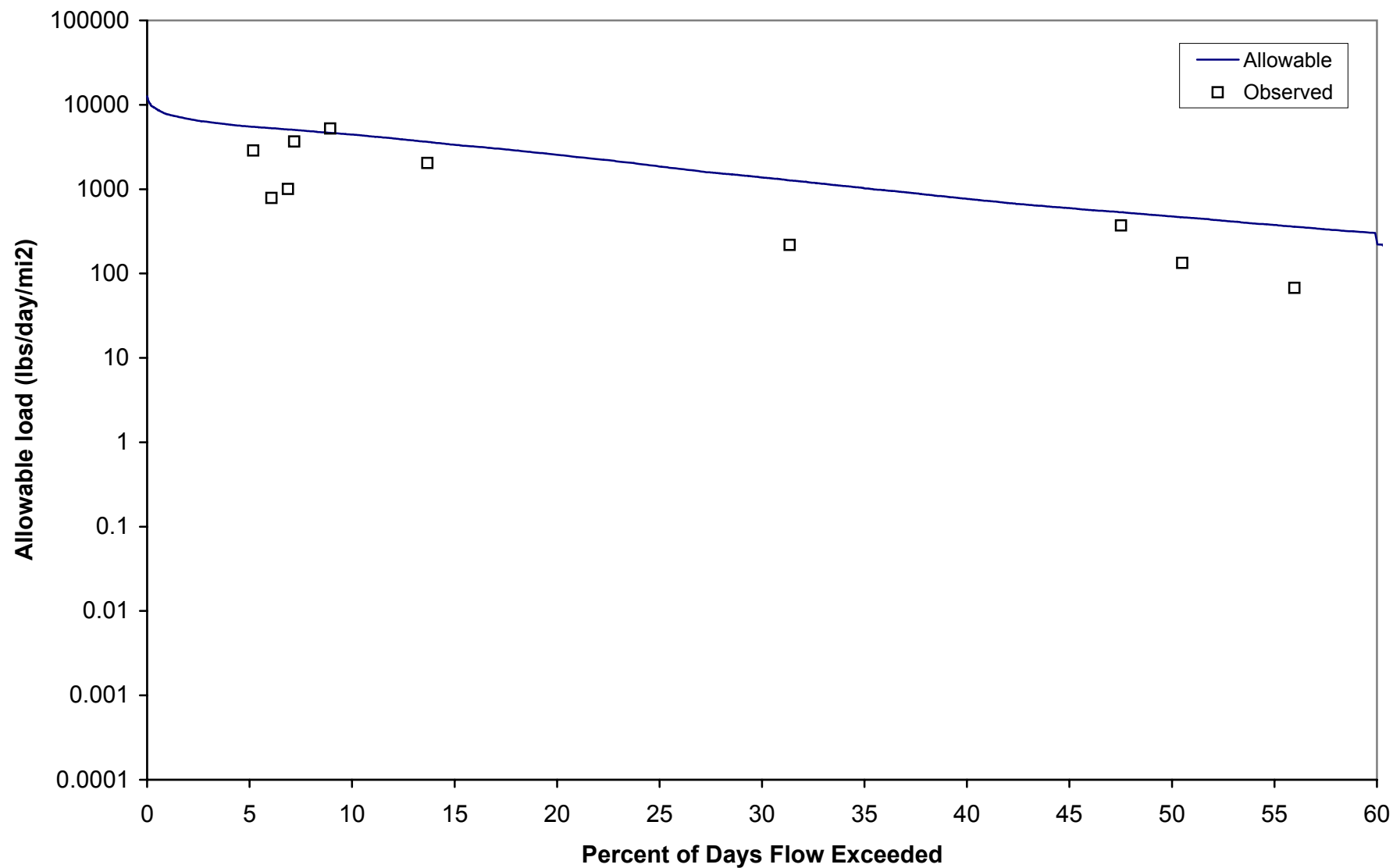
Figure F.2. Storm-flow Load Duration Curve for Village Creek (VGC0001)
